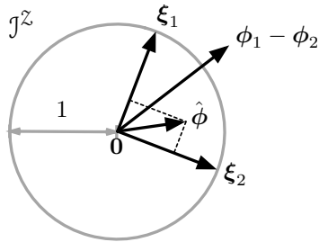
Fig. 1: The local geometry of decision making for distinguishing i.i.d. samples z^m over alphabet \mathcal{Z} from one of P_1, P_2 \in \mathcal{P}^{\mathcal{Z}} based on a statistic \ell = (1/m) \sum_{i=1}^m h^k(z_i) involving feature functions h^k . In information space \mathcal{J}^{\mathcal{Z}}(P_0) , where the reference distribution P_0 maps to the origin, \ell corresponds to the projection of the information vector \hat{\phi} for \hat{P} onto subspace spanned by the feature vectors \xi^k for h^k . The optimum decision rule projects \hat{\phi} directly onto \phi_1 - \phi_2 , the feature vector associated with the log-likelihood ratio h_{\text{LLR}} .
