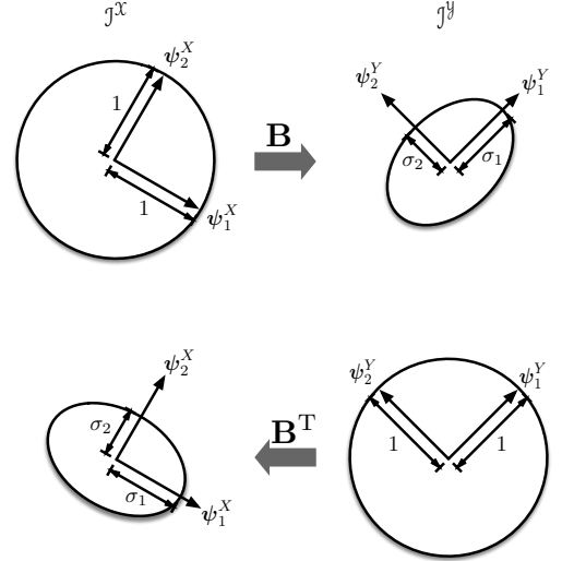
Fig. 2: The information geometry associated with the DTM \mathbf{B} . For i = 1, \dots, K-1 , the unit information vector \psi_i^X in \mathcal{P}^X maps via \mathbf{B} to the shorter information vector \sigma_i \psi_i^Y in \mathcal{P}^Y , and the unit information vector \psi_i^Y in \mathcal{P}^Y maps via \mathbf{B}^T to the shorter information vector \sigma_i \psi_i^X in \mathcal{P}^X .
