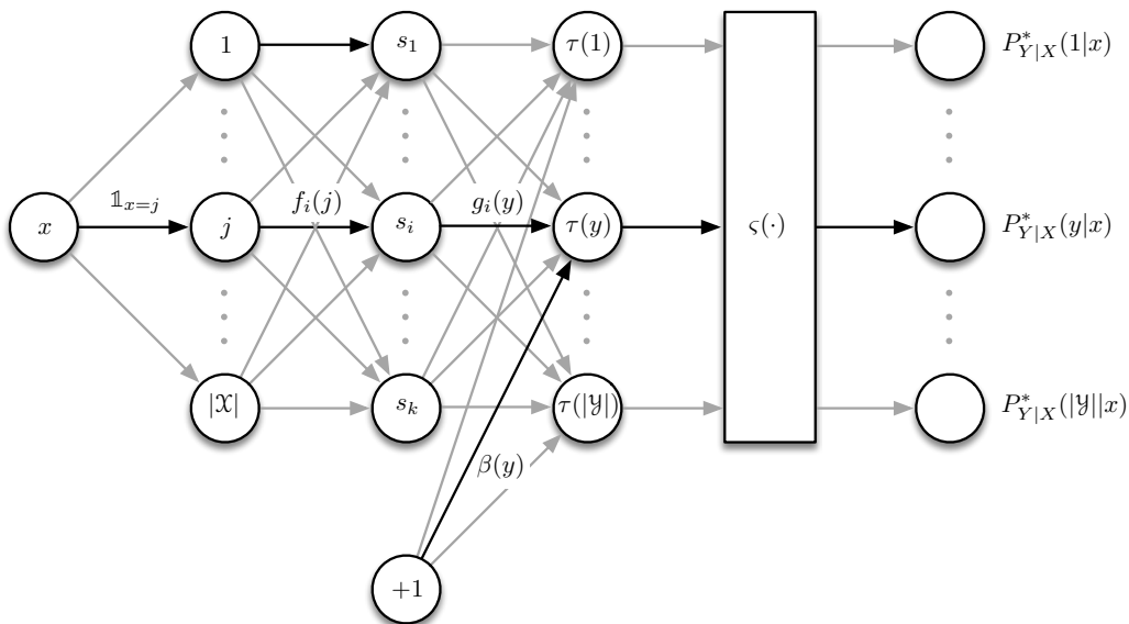
Fig. 3: A neural network representation of our softmax regression framework. In this network, we use a one-hot representation of the input x , corresponding to the kronecker weights \mathbb{1}_{x=j} . The hidden layer is characterized by the feature weights f_i(j) for i \in \{1, \dots, k\} , j \in \{1, \dots, |\mathcal{X}|\} , and the output layer is parameterized by the weights g_i(y) and biases \beta(y) , for i \in \{1, \dots, k\} , y \in \{1, \dots, |\mathcal{Y}|\} . The softmax processing, as defined in (236), is represented by the sigmoid function \zeta(\cdot) and operates on the unnormalized log-posterior \tau(y) .
