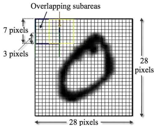
Fig. 4: Image representation for the preprocessing stage of the semi-supervised handwritten digit classifier. Each 28 \times 28 MNIST database image is decomposed into an array of 6 \times 6 = 36 subimages, each of size 7 \times 7 pixels, and each overlapping with its immediate neighbors by 3 pixels, horizontally and/or vertically.
