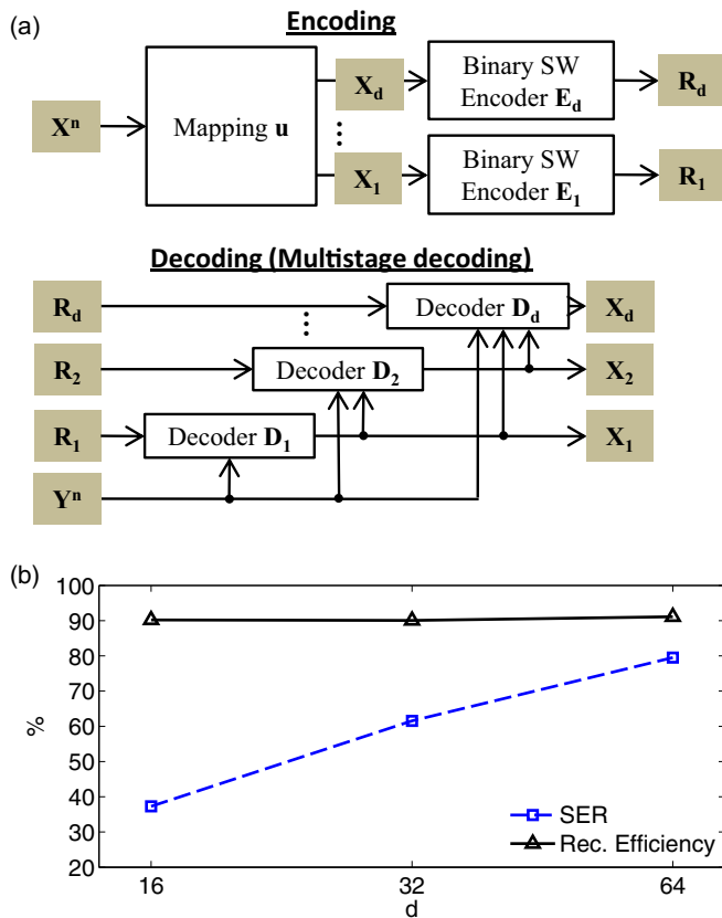
FIG. 3. (Color online) (a) Multilayer reconciliation scheme. Alice generates a message \mathbf{R} by applying a binary Slepian-Wolf code to each bit layer X_i , 1 \leq i \leq d , for each character in her sifted key \mathbf{X} . Bob receives \mathbf{R} and tries to recover each layer X_i , based on \mathbf{R} and his sifted key \mathbf{Y} [34]. (b) Experimentally obtained symbol-error rate (SER) and corresponding reconciliation efficiency \beta for different values of d at a photon pair generation rate of 0.28 pairs/pulse.
