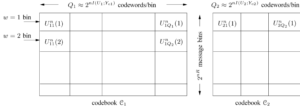
Fig. 3. Binning encoder for the secure product broadcast channel, for the case of M = 2 subchannels. The set of codewords for representing a particular message w \in \{1, \dots, 2^{nR}\} in the m th subchannel are denoted by U_{m1}^n(w), \dots, U_{mQ_m}^n(w) . To encode a particular message w , the encoder randomly selects one of the Q_m codewords in the associated bin for transmission in the m th subchannel, for m = 1, \dots, M .
