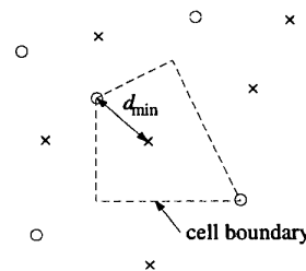
Figure 2: Quantization index modulation. The reconstruction points marked with \times 's and \circ 's belong to two different quantizers. The minimum distance d_{\min} measures the robustness to noise, and the sizes of the quantization cells determine the embedding-induced distortion.
