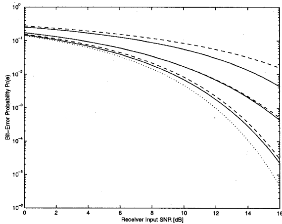
Figure 4: System performance with optimal and suboptimal transmitter power allocation. The successively lower solid curves correspond to the optimal bit-error performance of QPSK signaling for fading channels with coherence times \tau = 10, 1000, and 100000 symbols, respectively. The successively lower dashed curves denote the associated bit-error rates with the fixed power allocation \mathcal{E}_p/\mathcal{E} = 0.15 . Finally, the dotted curve depicts the bit-error probability for the case in which the channel is perfectly known.
