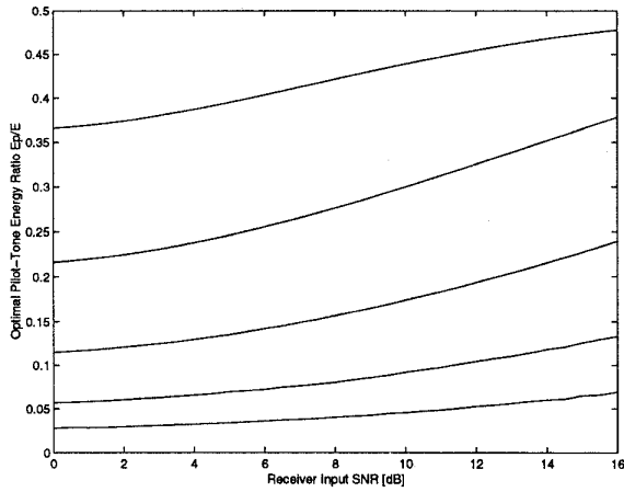
Figure 3: Optimal pilot-tone energy ratio \mathcal{E}_p/\mathcal{E} versus receiver input SNR. The successively lower curves correspond to fading channels with coherence times \tau = 10, 100, 1000, 10000, and 100000 symbols, respectively.
