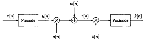
Figure 1: Narrowband spread-response precoding system model.
