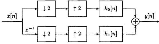
Figure 2: Filter bank structure of the linear, periodically time-varying spread-response precoder.
