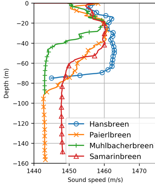
Figure 1-3: Representative depth-varying soundspeed profiles for underwater acoustic environments; in this case, different glacial bays in the same area (image reproduced with permission from [5]). Not only is the speed of sound highly variable with depth, but different bodies of water in the same geographical region can have large variations as well.
