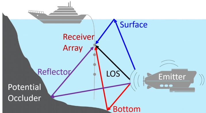
Figure 1-4: Typical shallow-water underwater acoustic localization problem setting; the image is modified from the original in [11]; licensed under a Creative Commons Attribution 4.0 International license.
