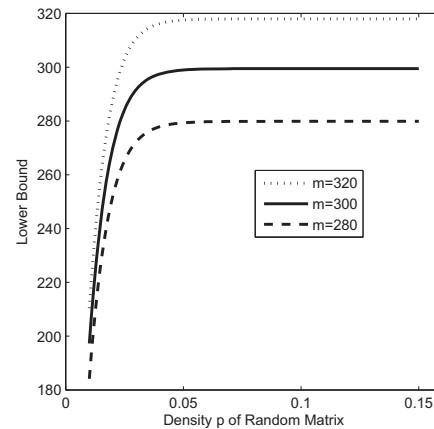
Fig. 2. The lower bound of H(Y|M, E, R) for the source described in Example 1.
