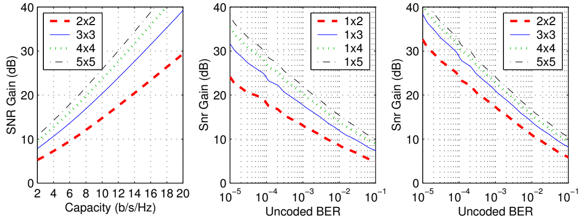
Figure 3-10: Achievable (left) and uncoded (middle, right, for 64-QAM) SNR gain for 1 \times N and N \times N systems for N = 2 to 5, relative to a 1 \times 1 system.
